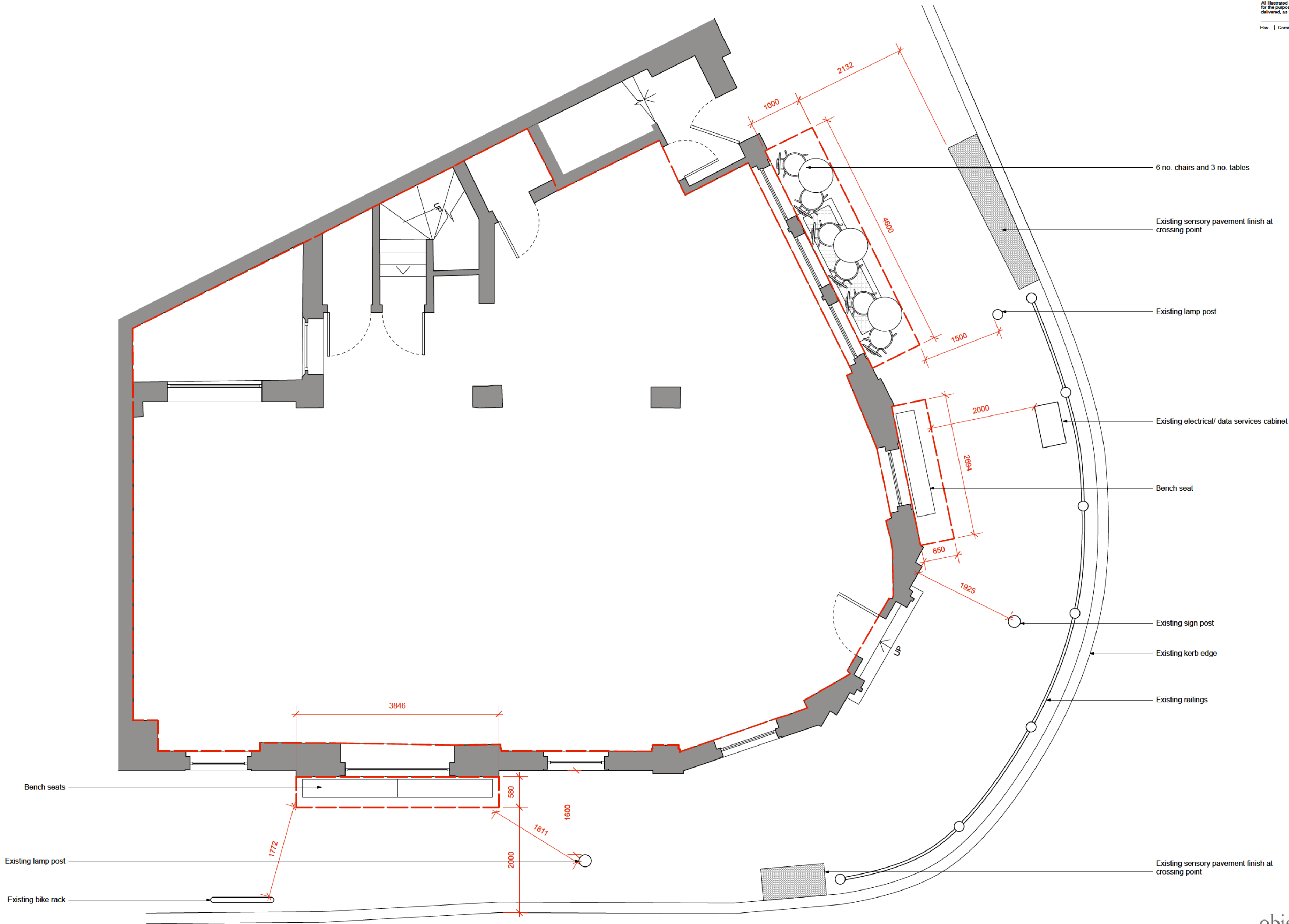
1 Proposed Pavement Plan Scale: 1:50
