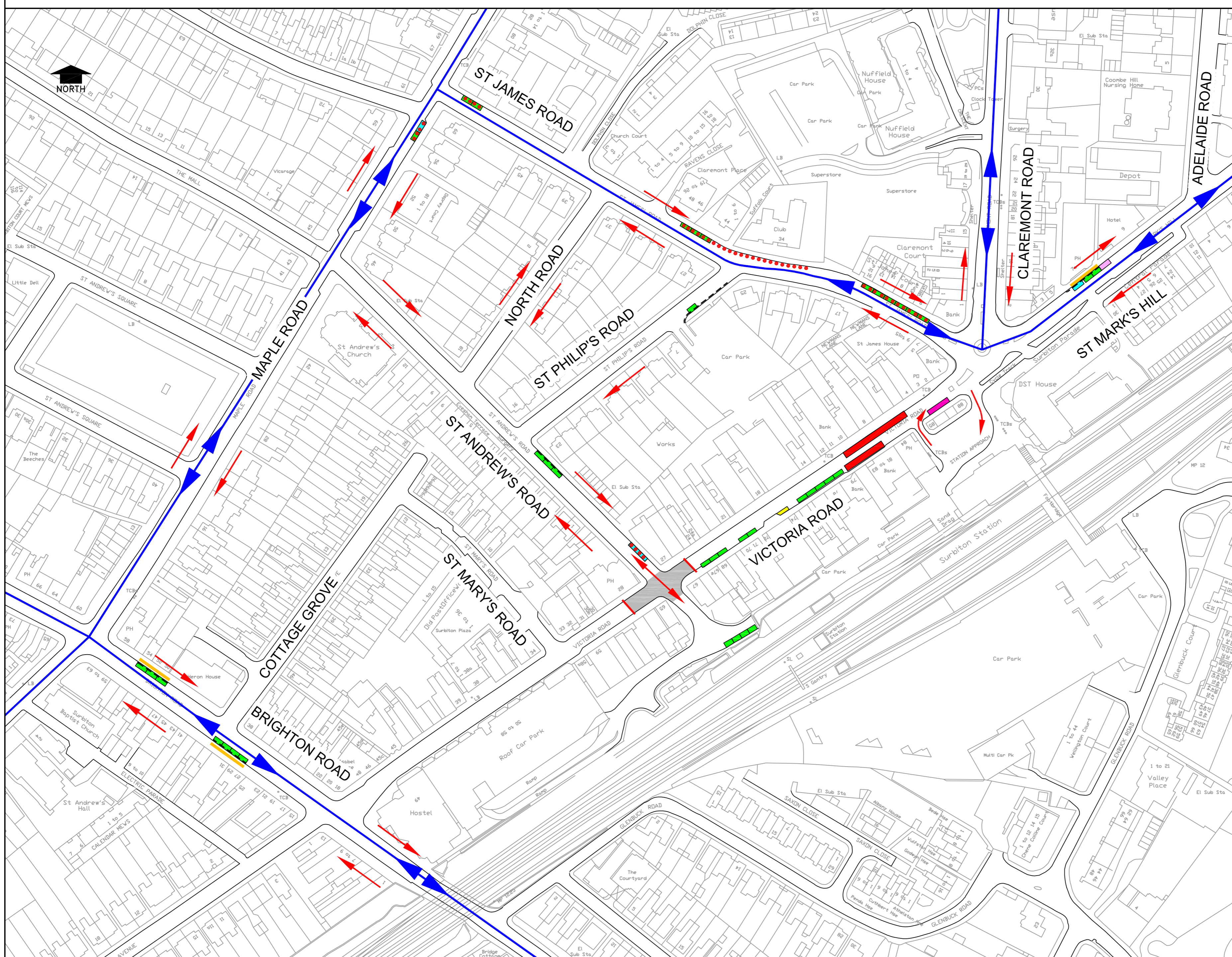
PLAN 2 – PROPOSED TRAFFIC FLOW DURING JUNCTION WORKS AT VICTORIA ROAD / ST ANDREW'S ROAD
