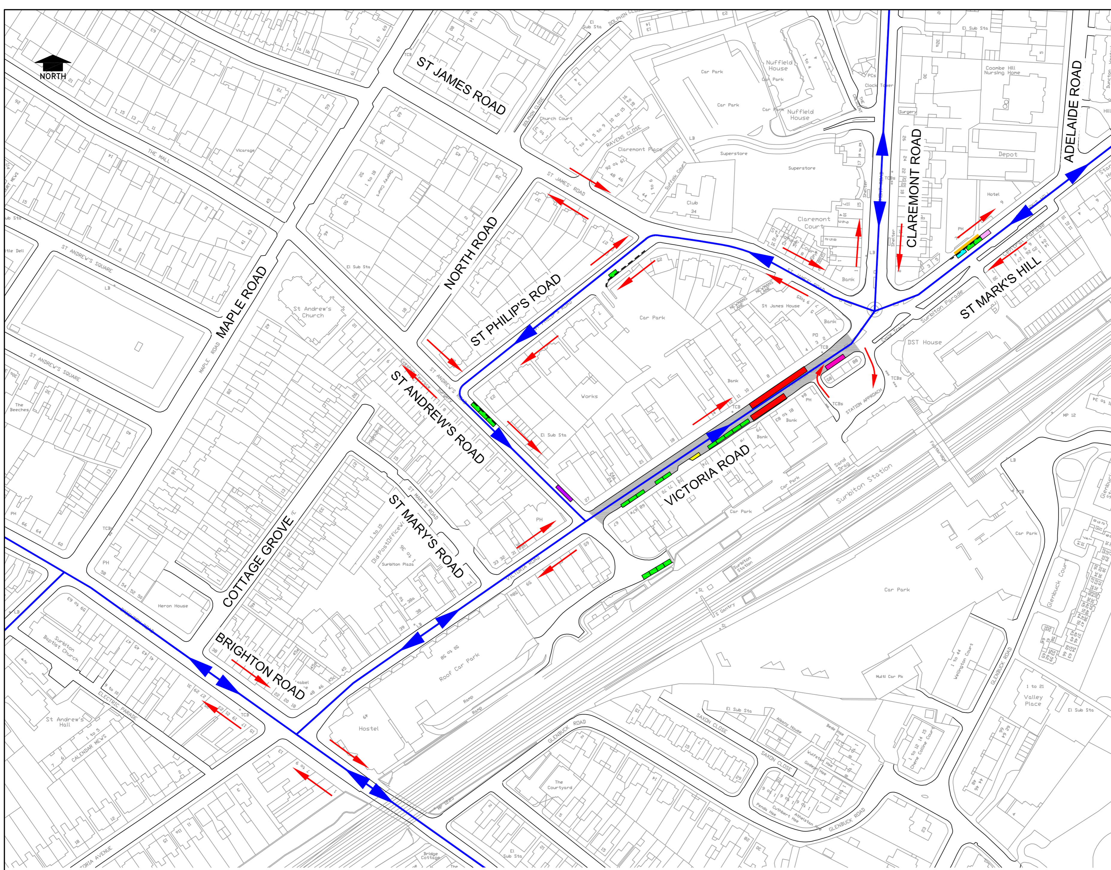
PLAN 1 – PROPOSED TRAFFIC FLOW DURING LANE CLOSURE IN VICTORIA ROAD
